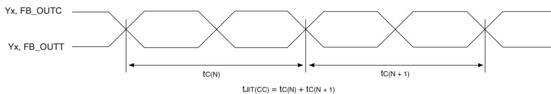
Figure 3: Cycle-to-Cycle Jitter
