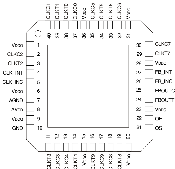
40-Pin MUF
