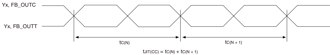
Figure 3: Cycle-to-Cycle Jitter
