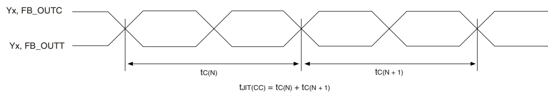
Figure 3: Cycle-to-Cycle Jitter
