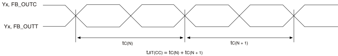
Figure 3: Cycle-to-Cycle Jitter
