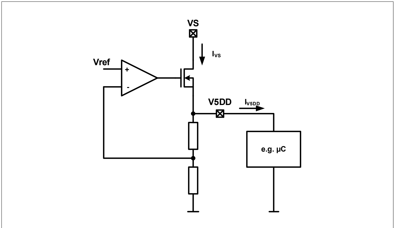
Figure 3 5V Supply
