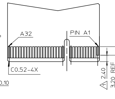
RECOMMENDED EDGE CARD PATTERN (SECONDARY SIDE) THICKNESS: 1.57mm
