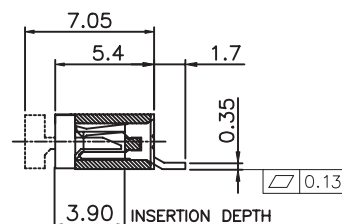
SECT. A-A
