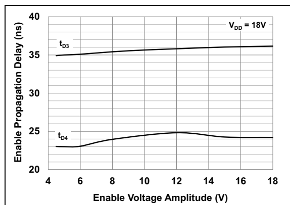
FIGURE 2-11: Enable Propagation Delay vs. Enable Voltage Amplitude.
