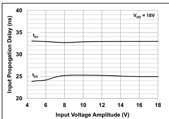
FIGURE 2-8: Input Propagation Delay vs. Input Amplitude.
