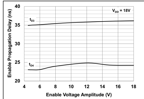
FIGURE 2-11: Enable Propagation Delay vs. Enable Voltage Amplitude.
