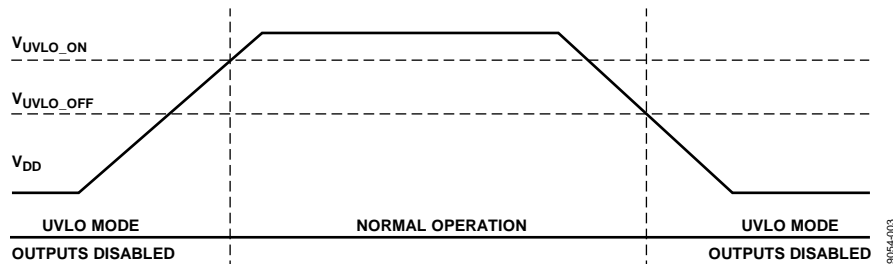
Figure 3. UVLO Function
