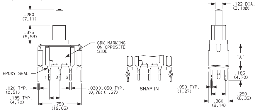
8161SH9_BE2 SPDT
