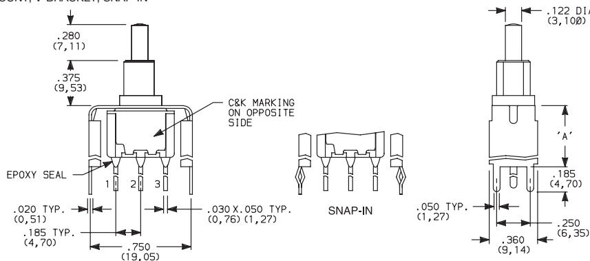
8161SH9_BE2 SPDT
