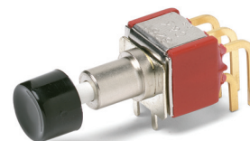
8261SH9ABE2 DPDT
