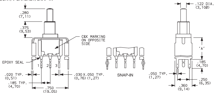
8161SH9_BE2 SPDT
