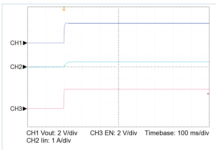
Figure 14 — Startup from EN, V_{IN} = 275\text{ V} , C_{OUT\_EXT} = 10000\text{ }\mu\text{F} , R_{LOAD} = 0.099\text{ }\Omega
