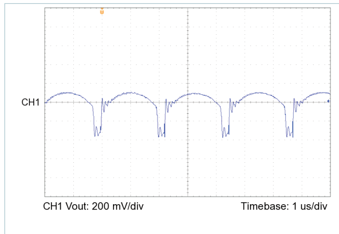
Figure 16 — Output voltage ripple, V_{IN} = 275\text{ V} , V_{OUT} = 3.3\text{ V} , C_{OUT\_EXT} = 1000\text{ }\mu\text{F} , R_{LOAD} = 0.099\text{ }\Omega
