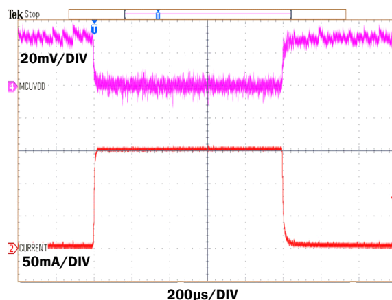
FIGURE 76. MCULDO LOAD TRANSIENT, I_{LOAD} = 0 TO 150mA, MCULDO OFFSET = 5.0V
