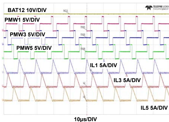
FIGURE 122. STEADY-STATE OPERATION (CURRENT) WAVEFORM IN BUCK/DE/NO-PD/LIGHT LOAD (5A)
