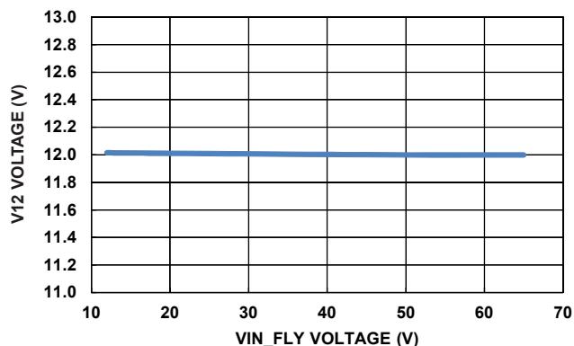
FIGURE 72. V12 LINE REGULATION, TEMP = +25°C, f_{SW} = 100kHz , V6 LOAD = 200 \Omega , V12 LOAD = 200mA
