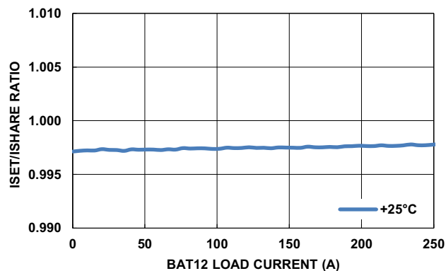
FIGURE 103. ISET/ISHARE RATIO vs LOAD CURRENT IN BUCK/DE/NO-PD
