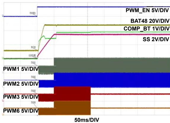
FIGURE 48. SOFT-START IN BOOST/FPWM/PD-ENABLED, 12V TO 48V, 6Ω LOAD ON BAT48
