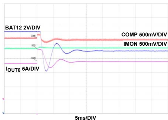
FIGURE 70A. RL1 = 0.15\Omega \rightarrow 0.1\Omega
