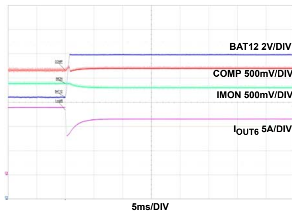
FIGURE 70B. RL = 0.10\Omega \rightarrow 0.15\Omega
