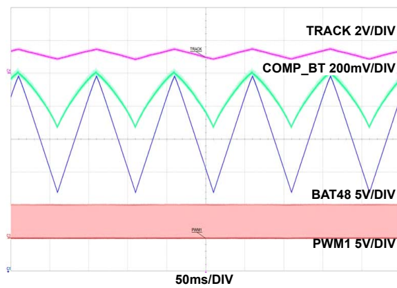
FIGURE 65. ANALOG TRACKING TRANSIENT WAVEFORMS IN BOOST/FPWM/NO-PD, A-TRACK SWEEP: 0.9V TO 1.5V, I_{OUT} = 20A
