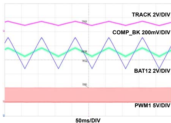
FIGURE 63. ANALOG TRACKING TRANSIENT WAVEFORMS IN BUCK/FPWM/NO-PD, A-TRACK SWEEP: 0.9V TO 1.5V, I_{OUT} = 100A
