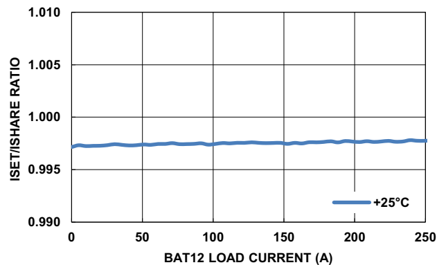
FIGURE 104. ISET/ISHARE RATIO vs LOAD CURRENT IN BUCK/FPWM/NO-PD
