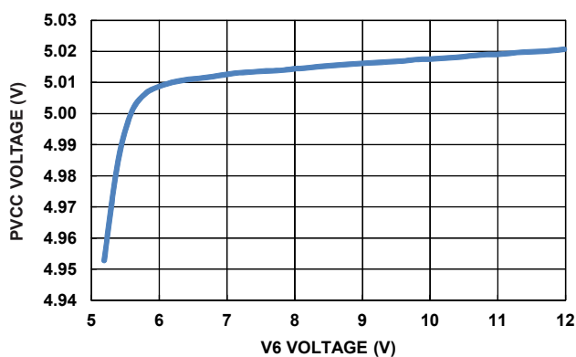
FIGURE 74. PVCC LDO LINE REGULATION, 0.2A \text{ LOAD}
