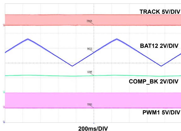
FIGURE 67. DIGITAL TRACKING TRANSIENT WAVEFORMS IN BUCK/FPWM/NO-PD, D-TRACK DUTY SWEEP: 40% TO 60%, F-DIGITAL TRACKING = 400kHz, I_{OUT} = 100A
