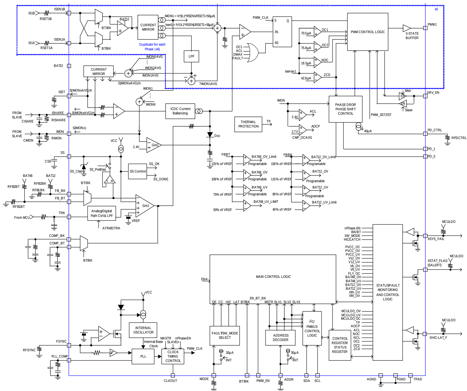
FIGURE 4. BLOCK DIAGRAM - BOTTOM
