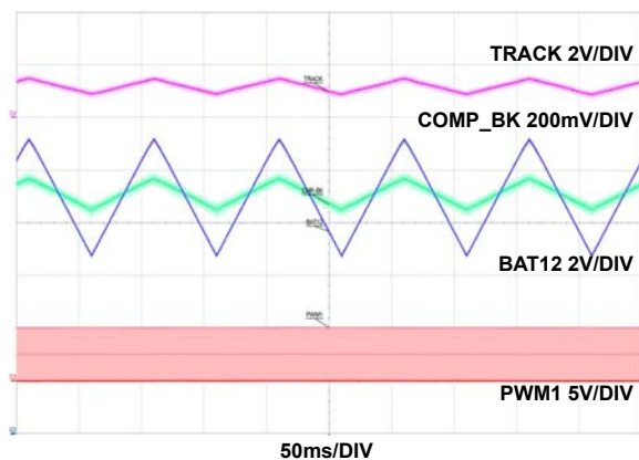
FIGURE 62. ANALOG TRACKING TRANSIENT WAVEFORMS IN BUCK/DE/NO-PD, A-TRACK SWEEP: 0.9V TO 1.5V, I_{OUT} = 100A
