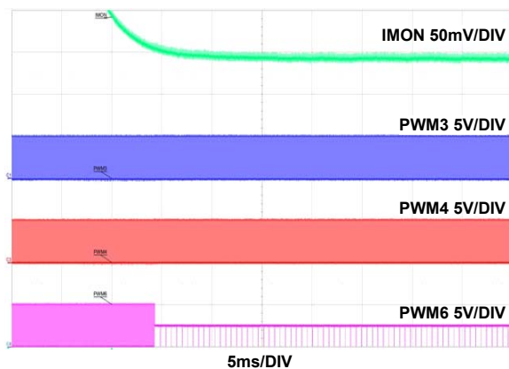
FIGURE 50. PHASE DROP TRANSITION IN BUCK/DE (6PH → 4PH), I_O = 150A \rightarrow 95A
