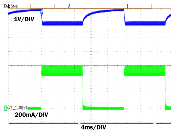
FIGURE 80. V6 LOAD TRANSIENT, V12 = 9Ω, V6 CURRENT = 0mA TO 500mA
