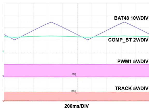
FIGURE 69. DIGITAL TRACKING TRANSIENT WAVEFORMS IN BOOST/FPWM/NO-PD, DIGITAL TRACKING DUTY SWEEP: 40% TO 60%, FREQUENCY-DIGITAL TRACKING = 400kHz, I_{OUT} = 20A
