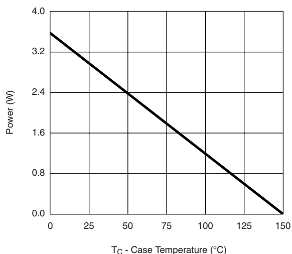
Power, Junction-to-Foot
