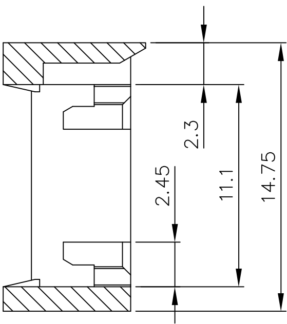
SECTION A-A Scale 5:1
