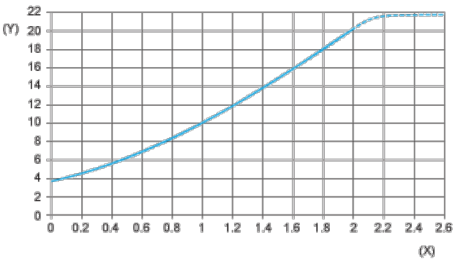
(Y) Is (mA) (X) Sensors - object distance (mm)
