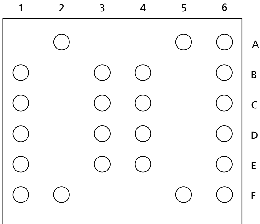
Figure 6: 23-Ball XFWLBGA (Top View)
