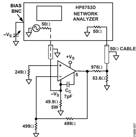
Figure 57. Negative PSRR
