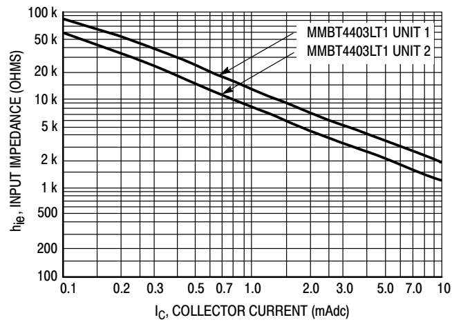
Figure 9. Input Impedance
