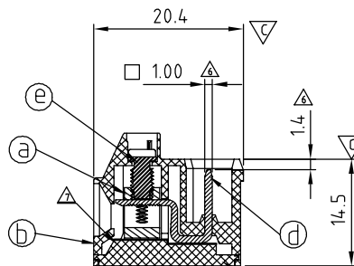
SECTION: P-P
