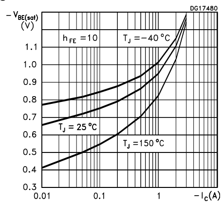
Figure 7. Base-emitter saturation voltage
