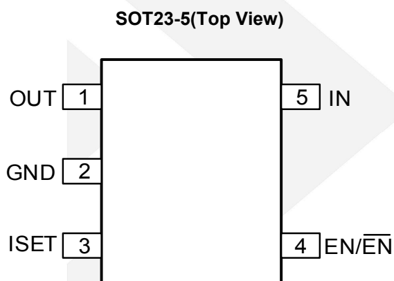
Figure 1 Pin Assignment
