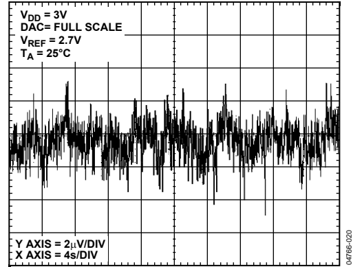
Figure 20. 0.1 Hz to 10 Hz Noise Plot
