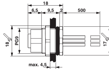
Dimensioned drawing
