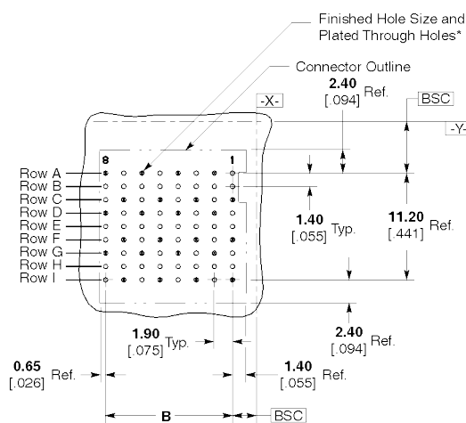
Recommended PC Board Layout Component Side Shown
