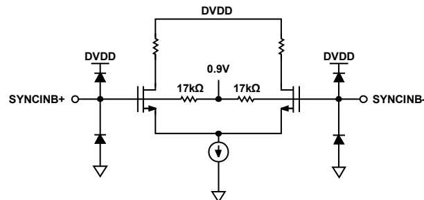
Figure 37. SYNCINB_{\pm} Circuit
