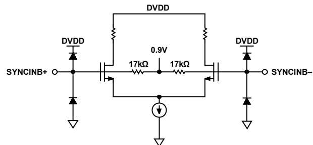
Figure 37. SYNCINB± Circuit
