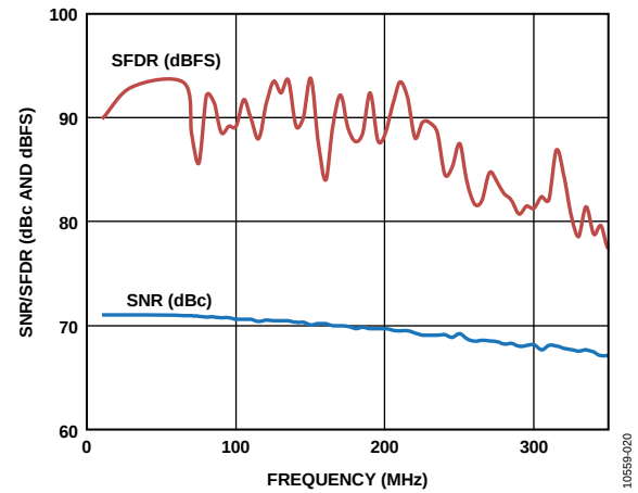
Figure 20. AD9250-250 Single-Tone SNR/SFDR vs. Input Frequency ( f_{IN} )
