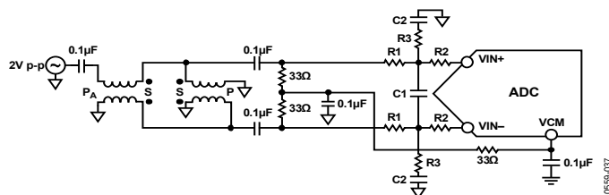
Figure 41. Differential Double Balun Input Configuration
