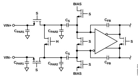
Figure 38. Switched-Capacitor Input
