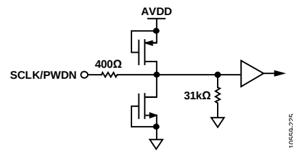
Figure 32. Equivalent SCLK or PDWN Input Circuit
