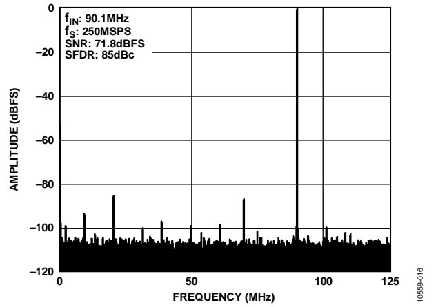
Figure 16. AD9250-250 Single-Tone FFT with f_{IN} = 90.1 MHz
