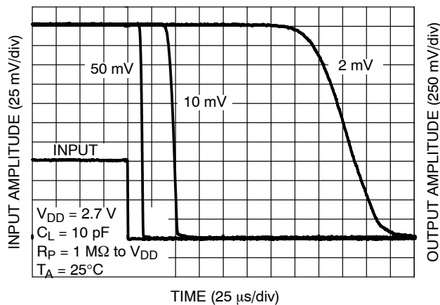
Figure 11. Propagation Delay H-L (2.7 V)
