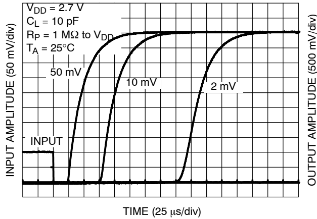
Figure 9. Propagation Delay L-H (5 V)
