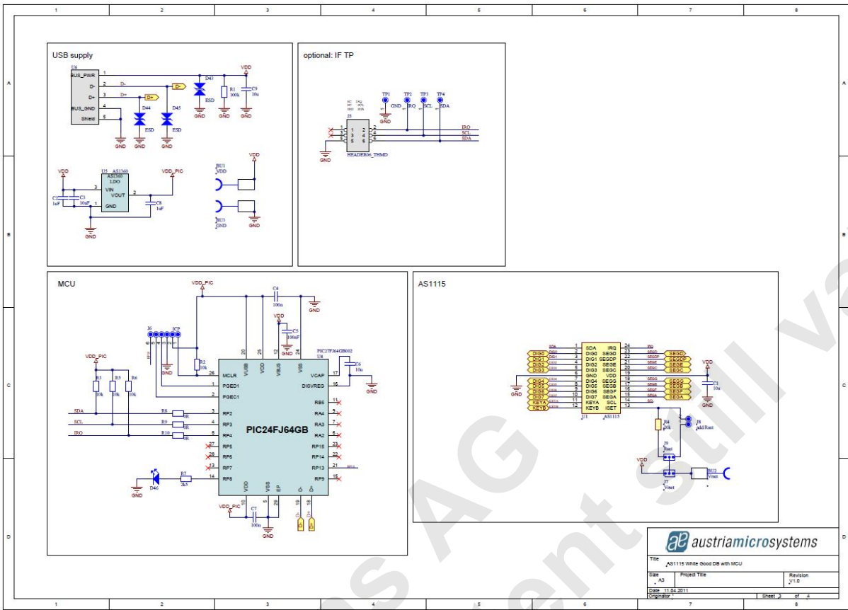
Figure 5: Main Schematic
