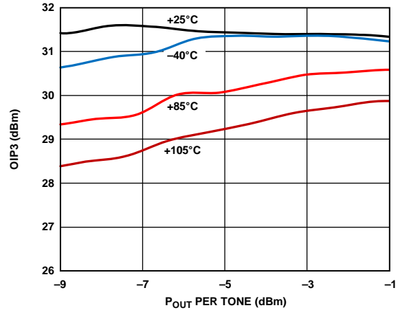
Figure 37. OIP3 vs. POUT at 30 MHz
