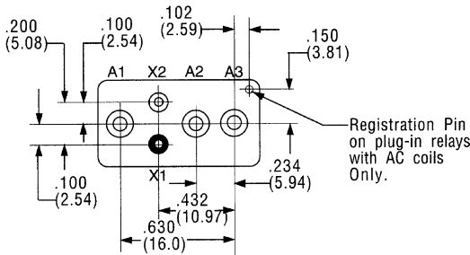
TERMINAL VIEW
