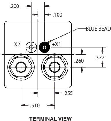
TERMINAL VIEW
