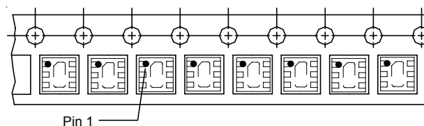
Device Orientation in Tape
