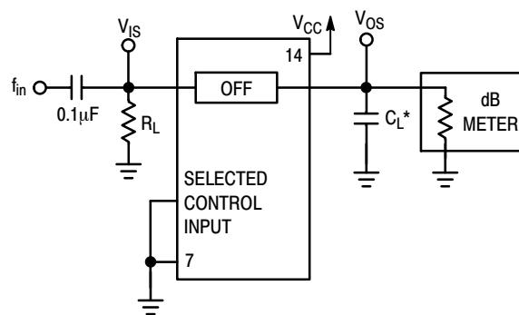
Figure 8. Off-Channel Feedthrough Isolation, Test Set-Up
