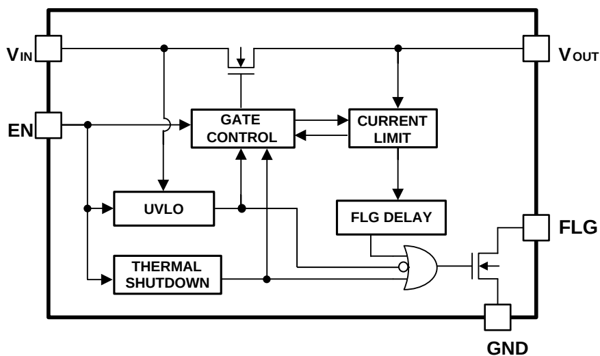
R5524xxxB Block Diagram
