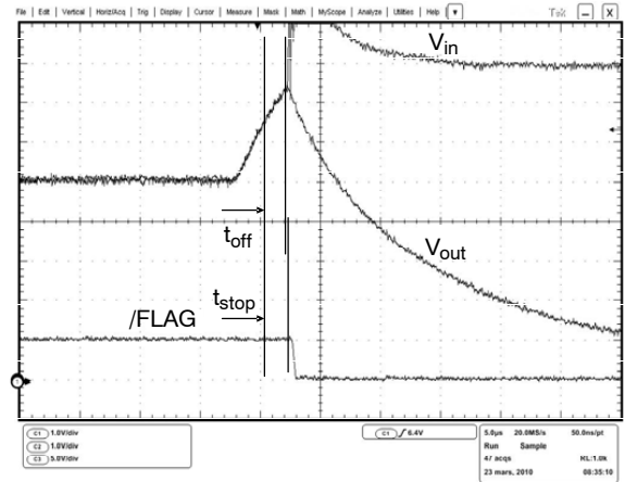
Figure 4. Overvoltage from 5 to 8 V, t_{off} and t_{stop}
