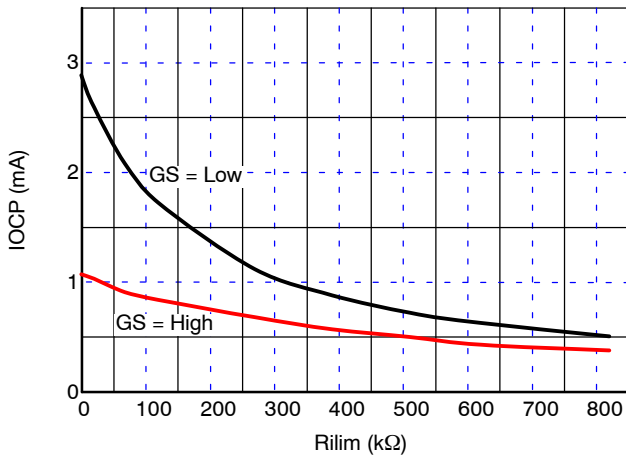
Figure 13. Over Current Threshold versus R_{LIMIT} 2.85 A Version
