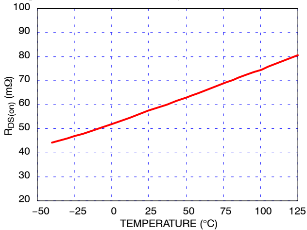
Figure 14. Typical R_{\text{DS(on)}} versus Temperature
