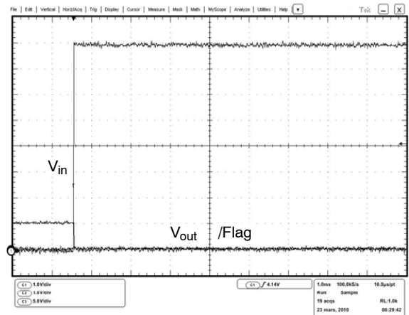
Figure 6. Overvoltage from 0 to 10 V
