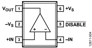
Figure 5. ADA4807-1 6-Lead SC70 Pin Configuration
