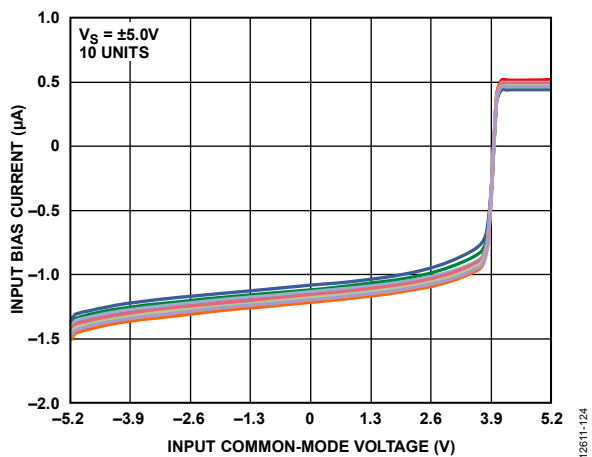
Figure 28. Input Bias Current vs. Input Common-Mode Voltage
