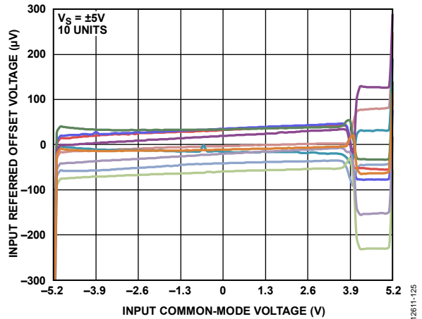
Figure 29. Input Referred Offset Voltage vs. Input Common-Mode Voltage
