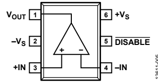
Figure 6. ADA4807-1 6-Lead SOT-23 Pin Configuration
