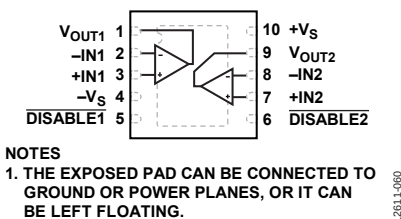
Figure 7. ADA4807-2 10-Lead LFCSP Pin Configuration
