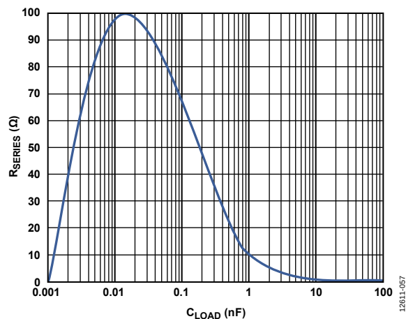
Figure 62. Required Series Resistor ( R_{\text{SERIES}} ) vs. Capacitive Load ( C_{\text{LOAD}} ) at 3 dB Peaking
