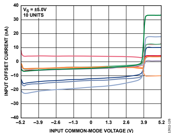
Figure 30. Input Offset Current vs. Input Common-Mode Voltage
