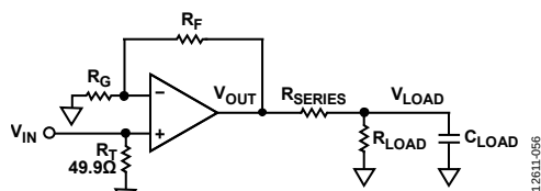
Figure 60. Schematic for Driving Large Capacitive Loads
