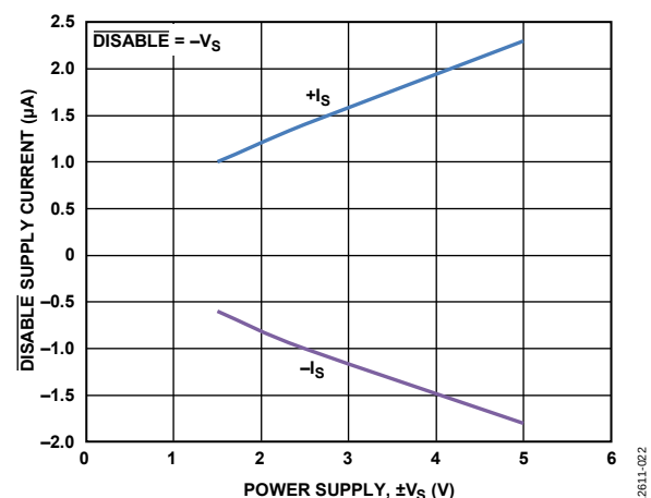
Figure 25. DISABLE Supply Current vs. Power Supply
