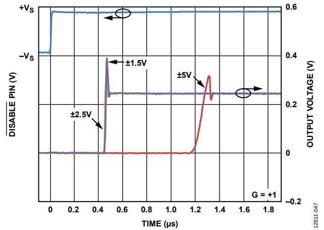
Figure 53. Power-Up Time for Various Supplies
