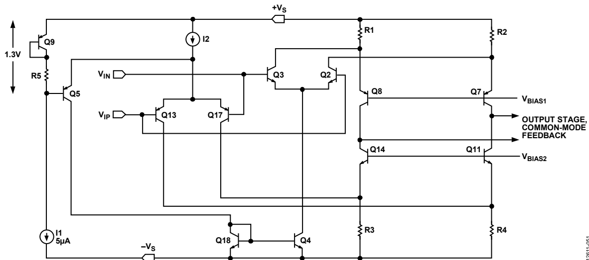
Figure 55. Simplified Schematic
