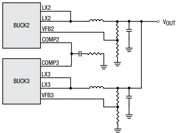
Figure 31. Parallel Operation
