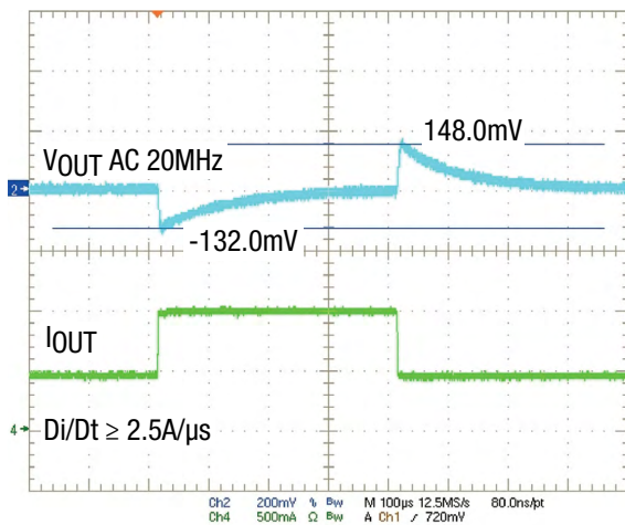
Figure 10. 12V IN , 3.3V OUT Transient Response, 0.5A to 1.0A
