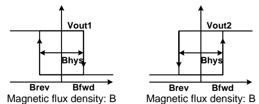
Figure 2. Output operation
