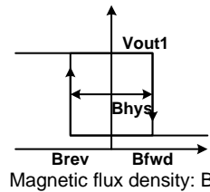
Figure 2. Output operation
