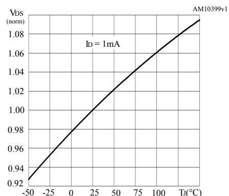
Figure 14. Normalized V_{(BR)DSS} vs temperature
