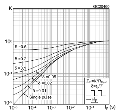
Figure 4. Thermal impedance for DPAK
