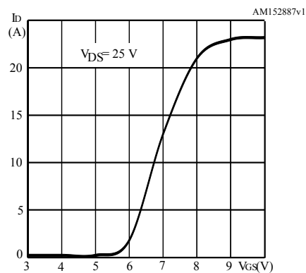
Figure 6. Transfer characteristics
