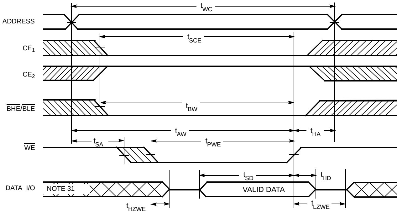
Figure 10. Write Cycle 4 ( \overline{\text{BHE/BLE}} Controlled, \overline{\text{OE}} LOW) [30, 32]
