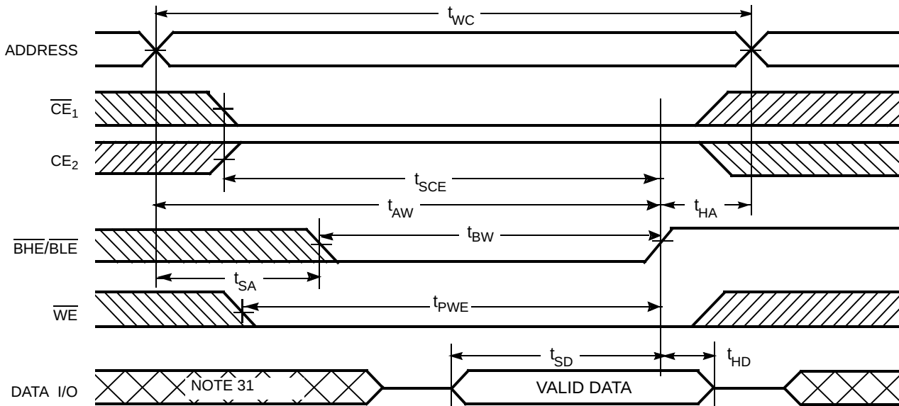
Figure 10. Write Cycle 4 ( \overline{\text{BHE/BLE}} Controlled, \overline{\text{OE}} LOW) [30, 32]
