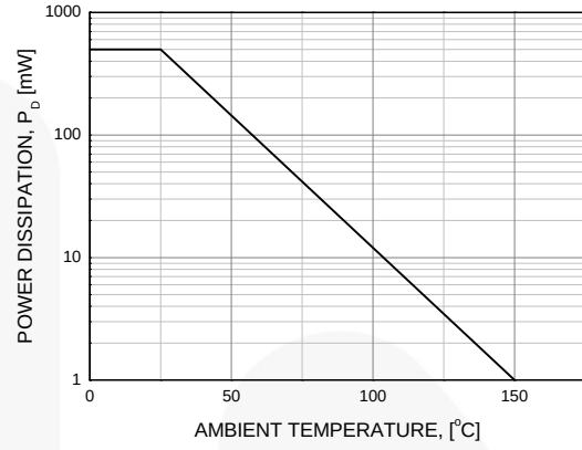
Figure 8. Power Deration
