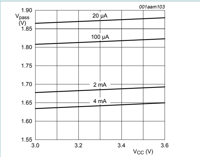
Fig. 8. Pass voltage versus supply voltage; T_{amb} = 85\text{ °C} (typical)
