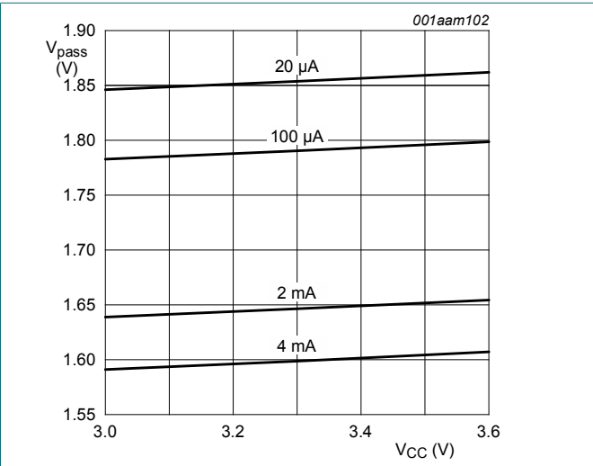
Fig. 7. Pass voltage versus supply voltage; T_{amb} = 125\text{ °C} (typical)
