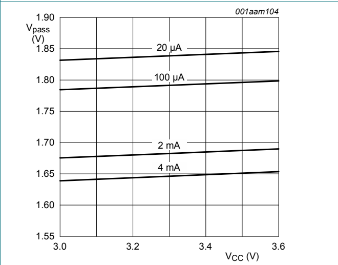
Fig. 9. Pass voltage versus supply voltage; T_{amb} = 25\text{ °C} (typical)
