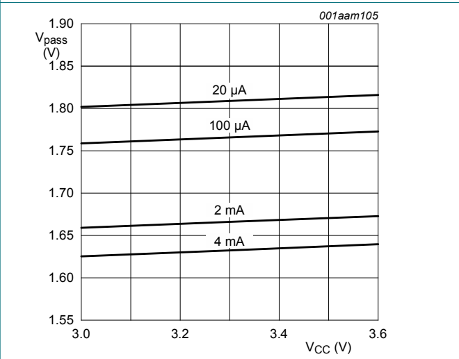
Fig. 10. Pass voltage versus supply voltage; T_{amb} = 0\text{ °C} (typical)
